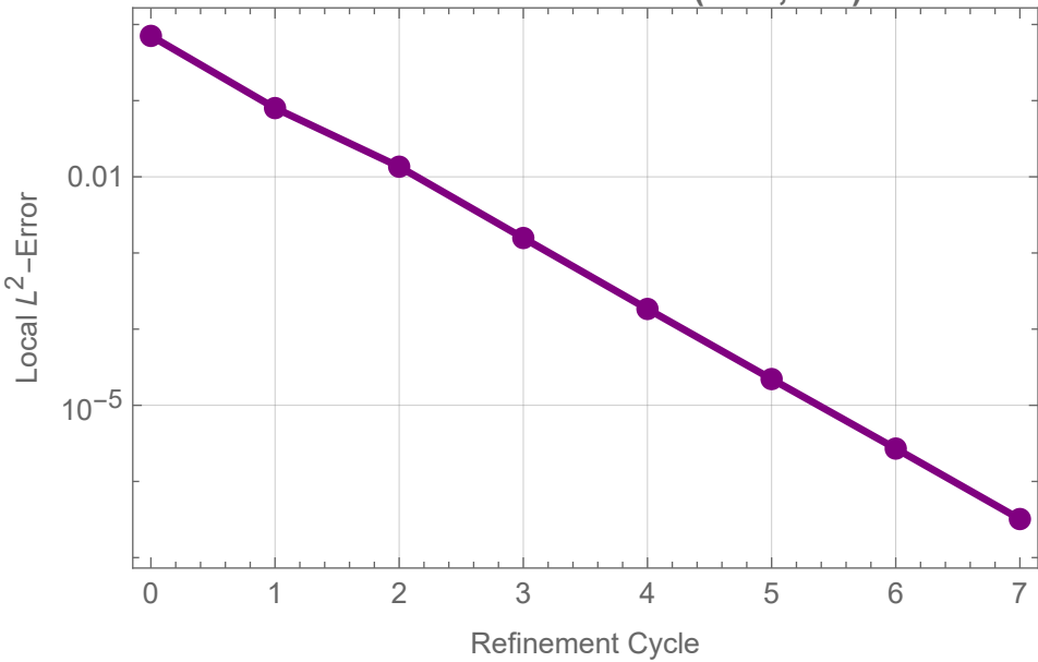
Local L^2 -Error at C = (0.75, 0.5)
